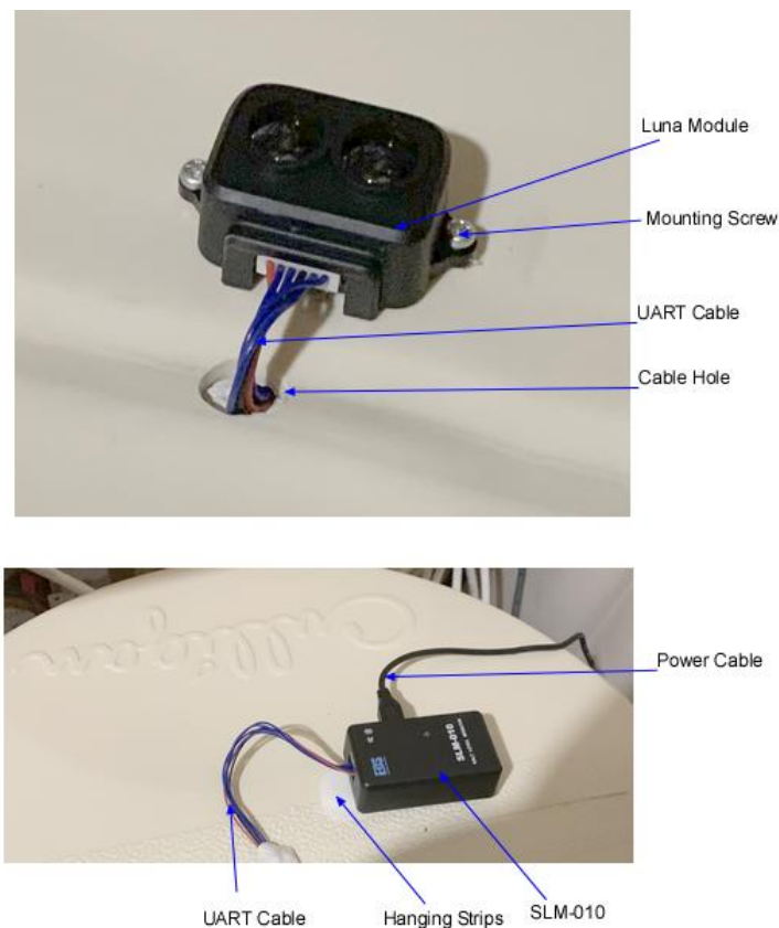
Figure 4 SLM-010 and Luna LiDAR Installation
