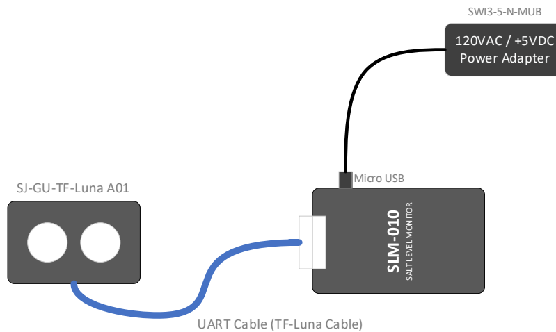
Figure 3 Connection Diagram
